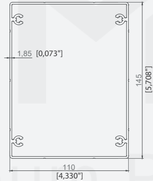
110x145 DİKME PROFİLİ 110x145 PILLAR PROFILE
