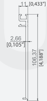
11X106,37 OLUK VE ARKA KAYIT KAPAÇI 11X106,37 GUTTER AND BACK BEAM COVER
