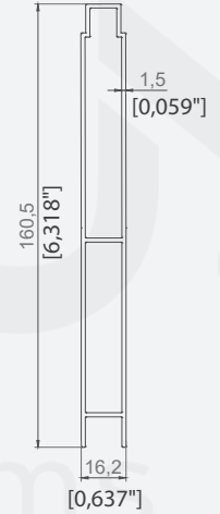
16,2X160 PANEL PROFİLİ 16,2X160 PANEL PROFILE
