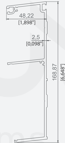
ARKA KAYIT PROFİLİ BACK BEAM PROFILE
