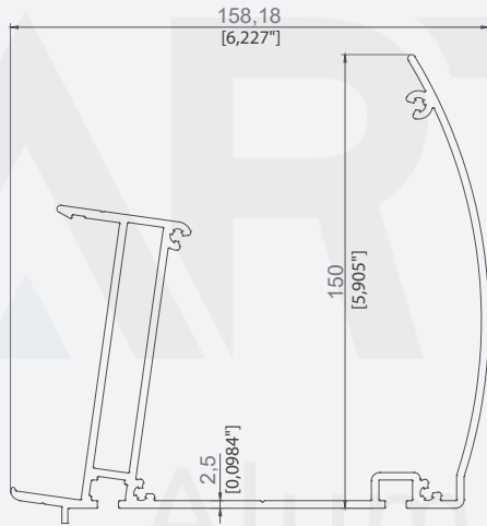
158X150 OVAL OLUK PROFİLİ 158X150 OVAL GUTTER PROFILE
