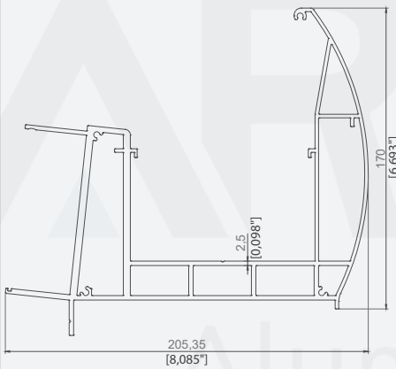
205X170 OVAL OLUK PROFİLİ 205X170 OVAL GUTTER PROFILE
