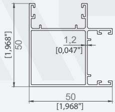
KÖŞE PANEL PROFİLİ CORNER PANEL PROFILE
