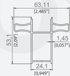
KULPLU PANEL PROFİLİ GLASS PANEL HANDLE PROFILE
