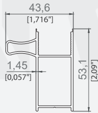
TEK KULPLU PANEL PROFİL GLASS PANEL SINGLE HANDLE PROFILE
