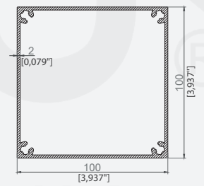
DİKME PROFİLİ PILLAR PROFILE
