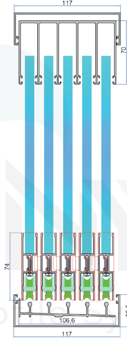
BEŞLİ CAM SİSTEMİ FIVE GLAZING SYSTEM
