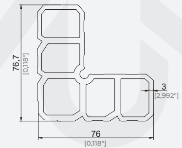
CAM PANEL KÖŞE TAKOZU PROFİLİ GLASS PANEL CORNER BLOCK PROFILE
