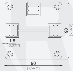
STANDART DİKME PROFİLİ STANDART PILLAR PROFILE
