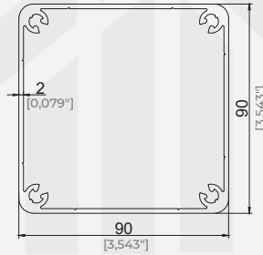
90x90 STANDART DİKME PROFİLİ 90x90 STANDART PILLAR PROFILE
