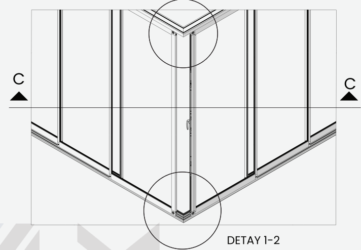
TEK YÖNE AÇILIR KAPI C DETAYINI GÖZETEREK İLERLEYELİM. LET'S PROCEED BY TAKING THE SINGLE-OPENING DOOR C DETAIL INTO CONSIDERATION.
